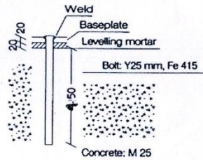
Anchor Bolt Detail
